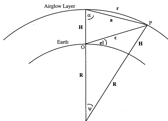
Fig. 6. Illustration showing airglow geometry.
