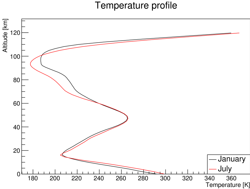
Figure 2.2: Temperature profiles of the atmosphere at latitude 30 °N created with the CIRA86 data for January and July. The biggest deviations can be observed in the mesosphere and MLT region.
