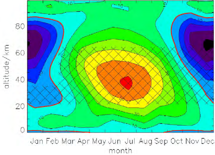
Figure 14: Mean zonal wind above Rothera from 0-100km. Generated from 6th order polynomial fits to the monthly mean data and, within the hatched area, monthly mean HWM-93 model winds. The thick red line represents the 0\text{ms}^{-1} contour, other contours are drawn at 10\text{ms}^{-1} intervals. Blue colour: westward winds. From (Hibbins et al. 2005)
