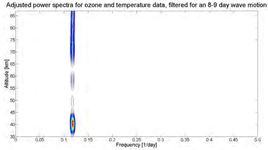
Figure 26: Power spectra for 8-9 day wave motions. In order to make both datasets visible, values from 35-75km have been divided by the mean of all values for ozone, and values at 87km by the mean of all values for temperature.
