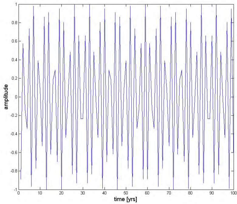
Figure 3-1 one wave with period close to the period pf the QBO, as one can see comes up a beating frequency even with when one wave is existing
