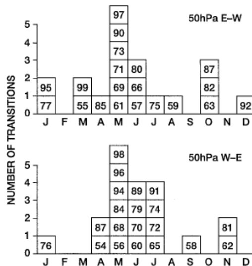
Figure 2-9 histograms of the number of zero crossings at 50 hPa grouped by month
