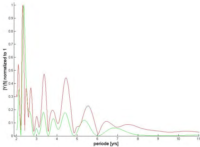
Figure 4-7-a In red is shown the cross spectrum between the planetary wave amplitudes, averaged over wave number and pressure level, and the QBO. Also shown in green is the FFT of the QBO
