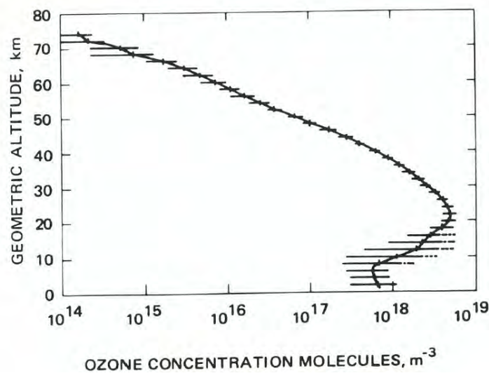
Figure 2-1 average ozone concentration over altitude for mid latitudes [Andrews, 2000]
