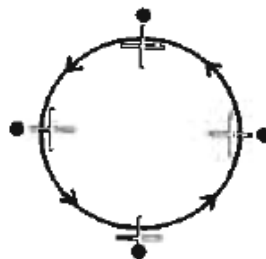
Figure 2-5 vorticity meter in a solid state rotation [Andrews, 2000]
