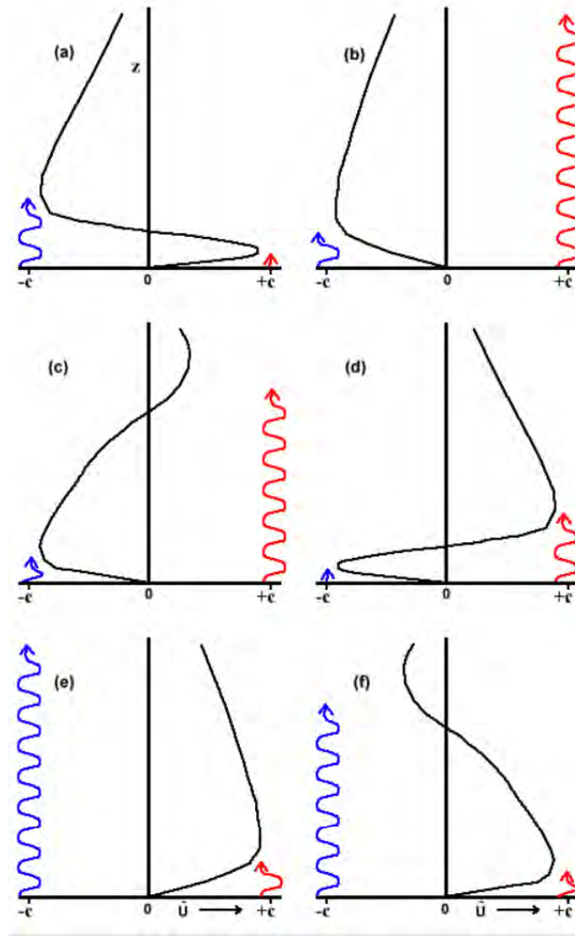
Figure 2-11 mechanism for the QBO [Plumb, 1977; Heaps, 2009]
