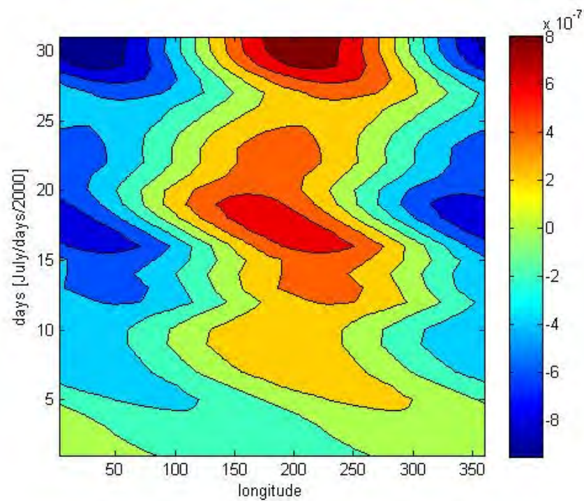
Figure 4-3 example for the reconstruction of PW data separated in wavelength fitted to the form A \cdot \cos(x) + B \cdot \sin(x) , reconstructed in the same form
