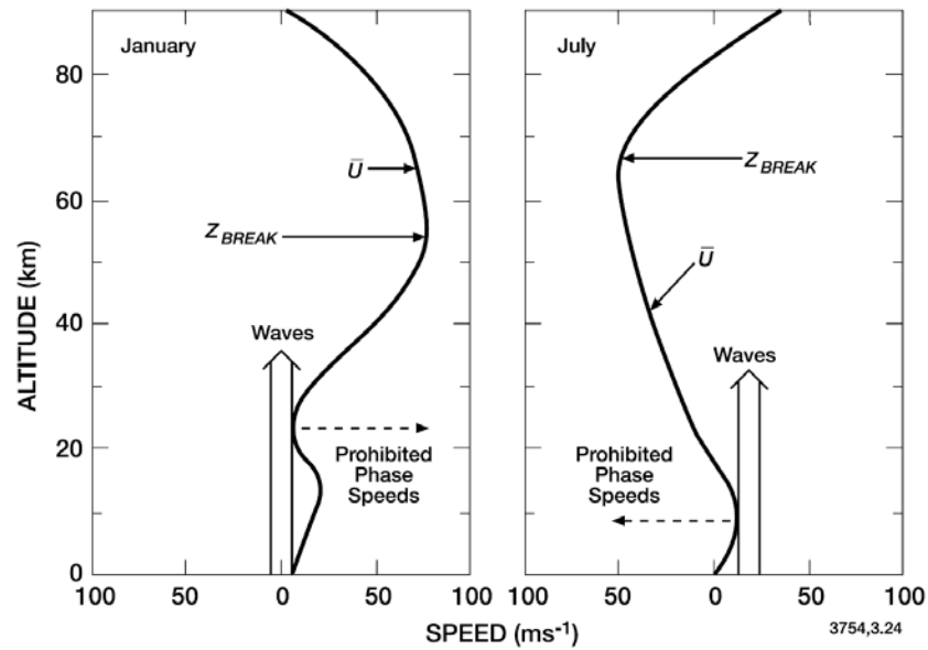
Figure 2-3 effect of the wind fields (e.g. the steady state wind fields) on the propagation of gravity waves [Brasseur and Salomon, 1984].
