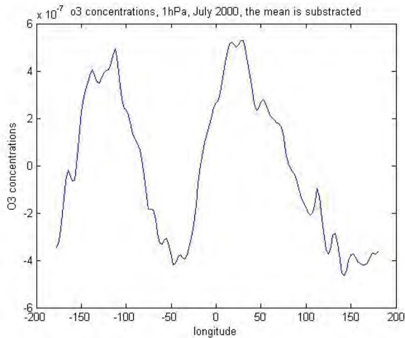
Figure 4-2 example of the ERA 40 data. The graph shows the O 3 -data -averaged over days and latitude- over longitude from the level of 1hPa from the 21. July 2000
