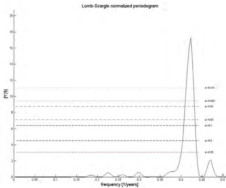
Figure 4-9-b lomb periodogram of the QBO for the pressure level 45hPa. One can clearly recognize the strong peak at 2.359 years
