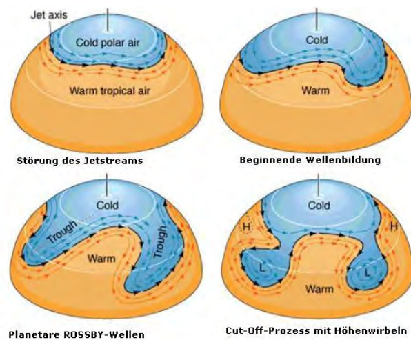
Figure 2-8 an amplifying PW with a detaching parcel of cold air [Boljahn, 2009]
