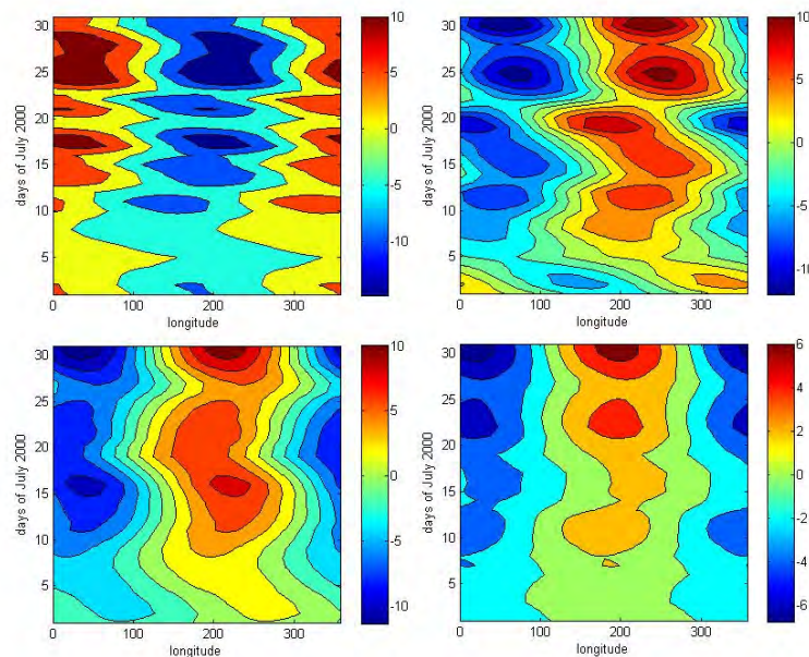
Figure 5-1 Hovmöller contour plots of wave number 1, altitudes are from the top left to the bottom right 1, 10, 50, 100 hPa for the temperature in July 2000
