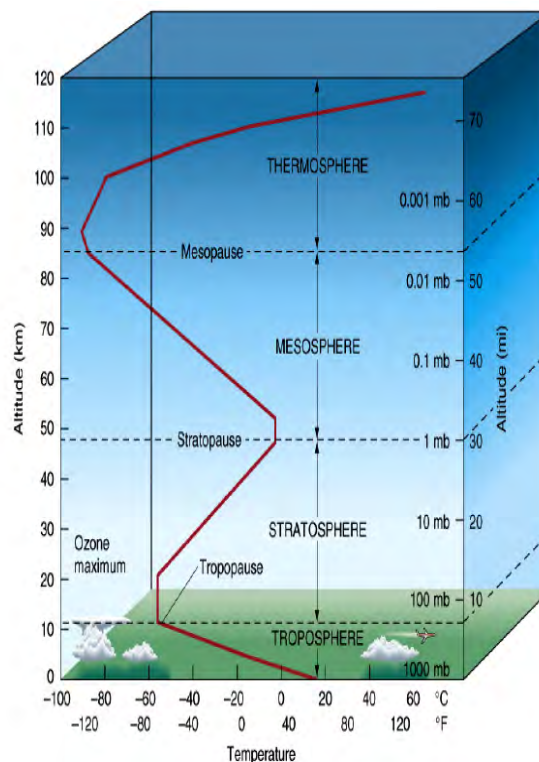
Figure 2-3 steady state of earths atmosphere with the division into layers. In the stratosphere is marked the maximum in ozone concentration
