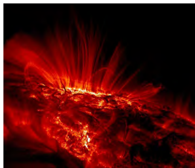
Figure 2-13 sunspot viewed in ultraviolet light [Nemiroff, 2002]
