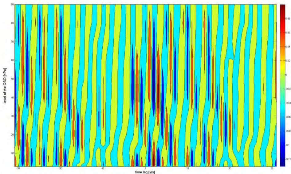
Figure 4-8 contour plot of the 3 waves fit from the xcov between the averaged PW amplitudes for the variable t and the QBO
