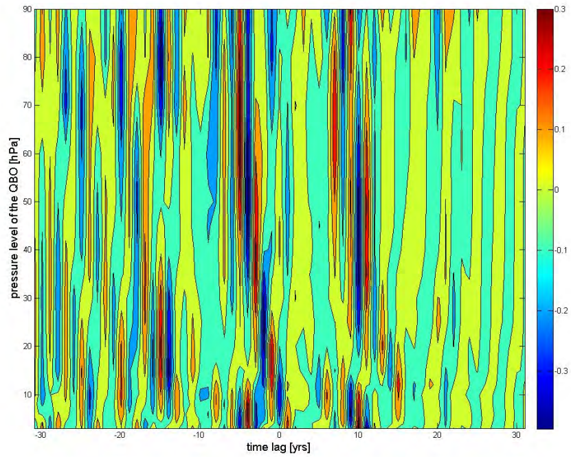
Figure 4-5 xcov between the QBO and the 10hPa PW amplitude of wavenumber 2. The few more than 2 years periode of the QBO is good visible but as well another period with about 10 to 15 years (between the red parts)
