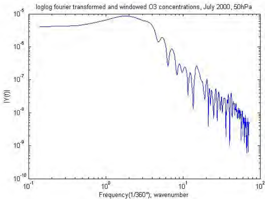
Figure 4-1 the windowed and fourier transformed O 3 concentration for July 2000
