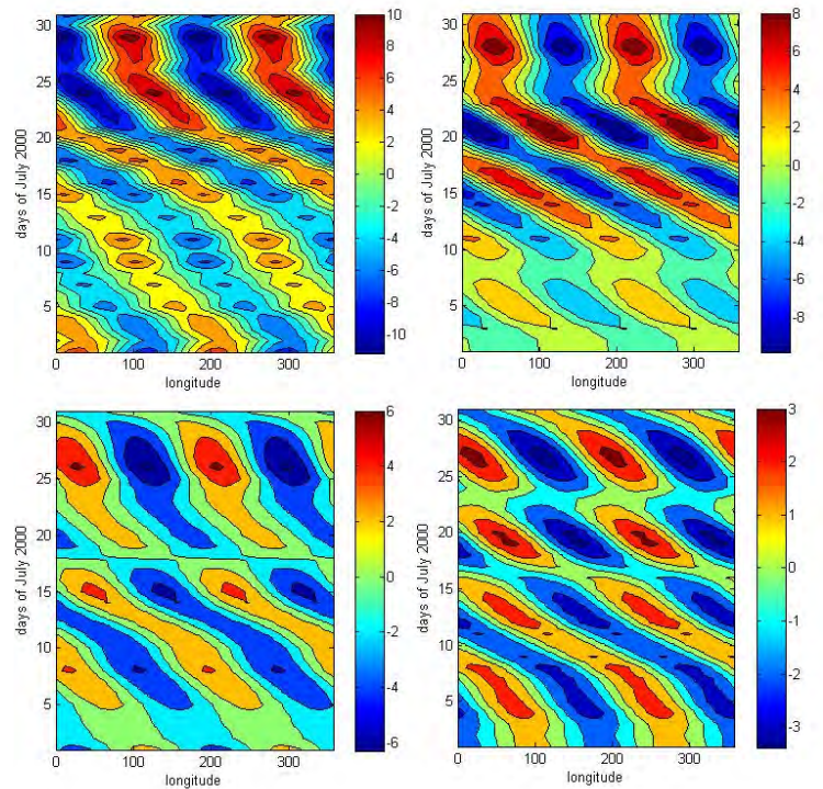
Figure 5-2 Hovmöller contour plots of wave number 2, altitudes are from the top left to the bottom right 1, 10, 50, 100 hPa for the temperature in July 2000
