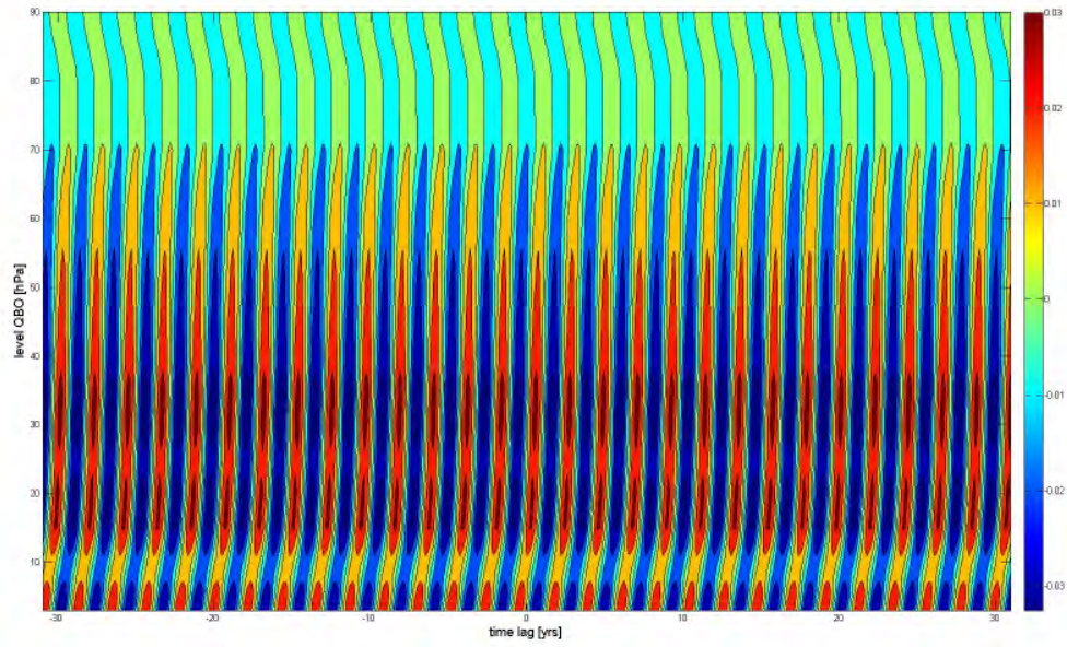
Figure 4-9 contour plot of the one wave fit from the xcov between the averaged PW amplitudes for the variable t and the QBO
