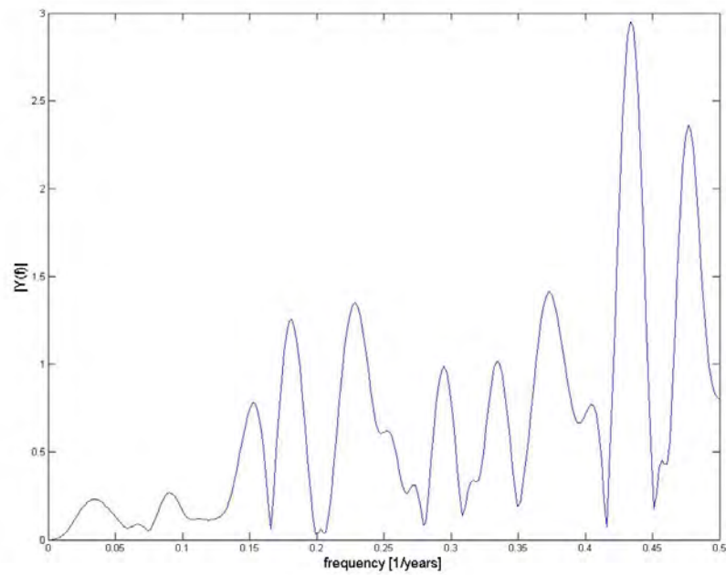
Figure 4-6 FFT of the xcov between the QBO at 40hPa and the PW of wave number 6 at 100hPa
