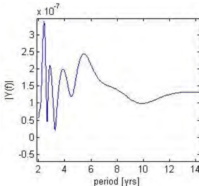
Figure 4-4 detail of the FFT of the PW amplitudes on the level 50hPa and of the wave number 3. One can clearly recognise a strong peak at about 2.4 years
