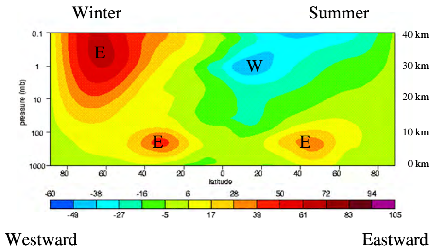
Figure 2-2 atmospherical wind field (without any wave activity) [ Espy, 2009 ]
