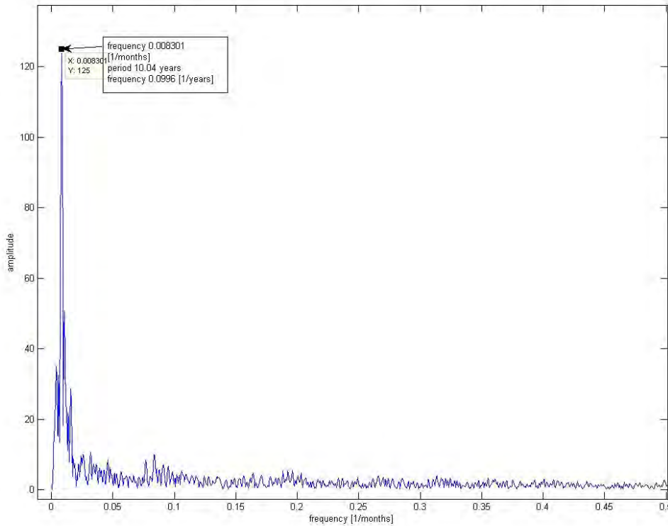
Figure 5-3 frequency spectrum of the F10.7 solar cycle documentation. One can clearly recognize the strongest peak at 0.0996 [yrs -1 ]
