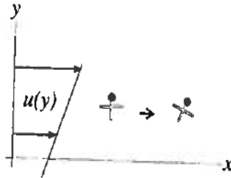
Figure 2-6 vorticity meter in a 2-dimensional shear flow [Andrews, 2000]
