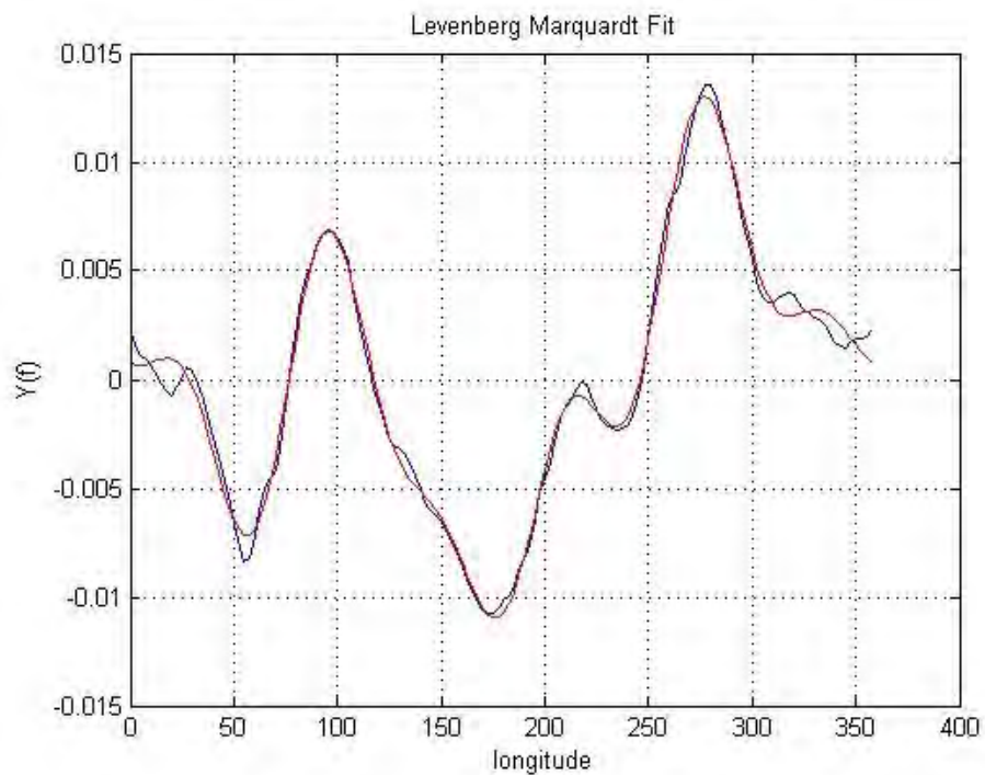
Figure 4-2 example for a Levenberg-Marquardt fit of the O 3 -concentration over longitude. The blue line gives back the original data and the red line the fitted data
