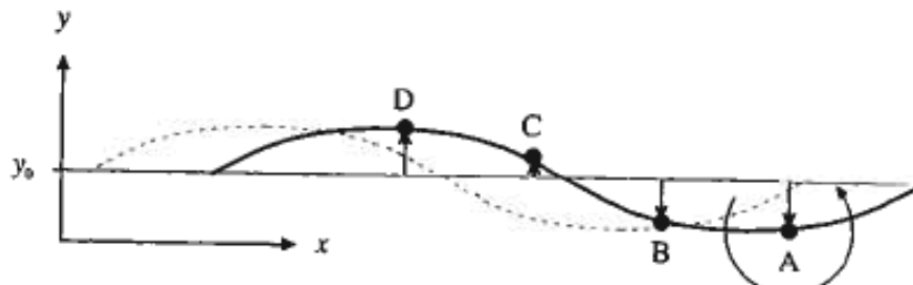
Figure 2-7 simplified 2-dimensional PW mechanism, in terms of conservation of potential vorticity [Andrews, 2000]
