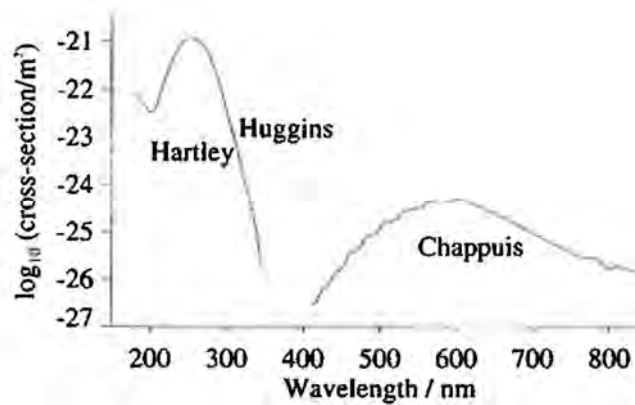
2-1 absorption cross section for O 3 [Andrews, 2000]
