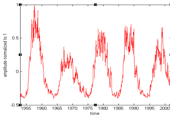
Figure 3-3 the F10.7 radio flux monthly average
