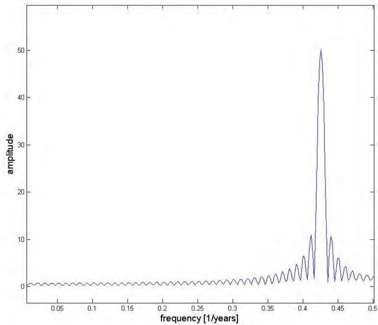
Figure 3-2 FFT of the data plotted in figure (3-1). There is only one single peak existing, so the upcoming beating frequency is only visible in the plot and no modulation
