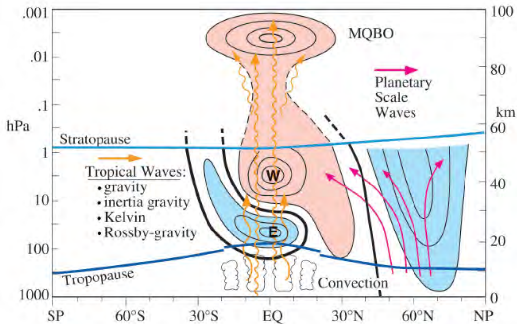
Figure 2-10 dynamical overview of the QBO during northern winter
