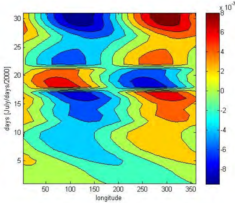
Figure 4-1 example for the phase shift under the reconstruction of PW data separated in wavelength fitted to the form A \cos(x) + B \sin(x) , reconstructed in the form C \cos(x + \phi)
