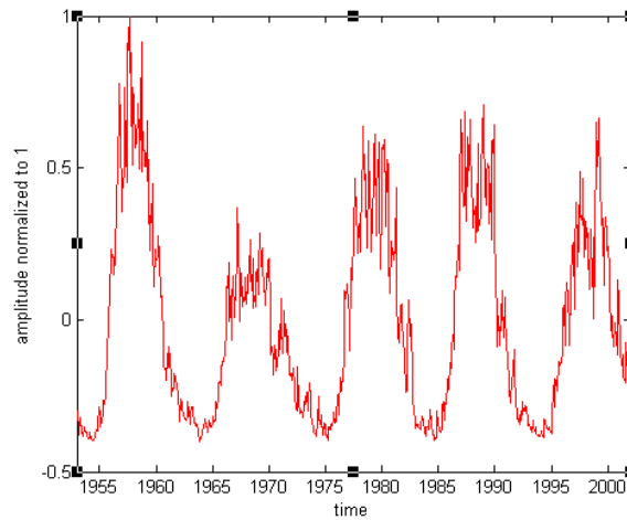
Figure 2-14 the monthly averaged F10.7 radio flux
