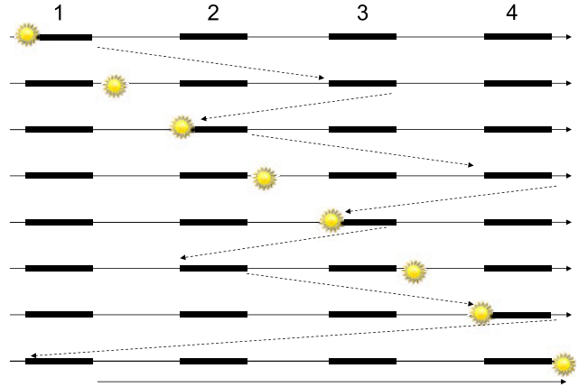
Figure 6. The flux determination procedure. Each of the stacked horizontal lines depicts the segment of the solar track containing four arcs. Time increases downward. The set of arcs spans about 15^\circ .
