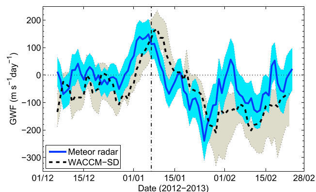
Figure 4. Ten day moving average GWF (in \text{m s}^{-1} \text{ day}^{-1} ) at 90 km over Trondheim, Norway, derived from meteor radar observations (blue, errors are shaded) and as simulated in WACCM-SD (black dashed line, area between maximum and minimum GWF in layer is shaded). Onset of the SSW is indicated by a black dash-dotted line.
